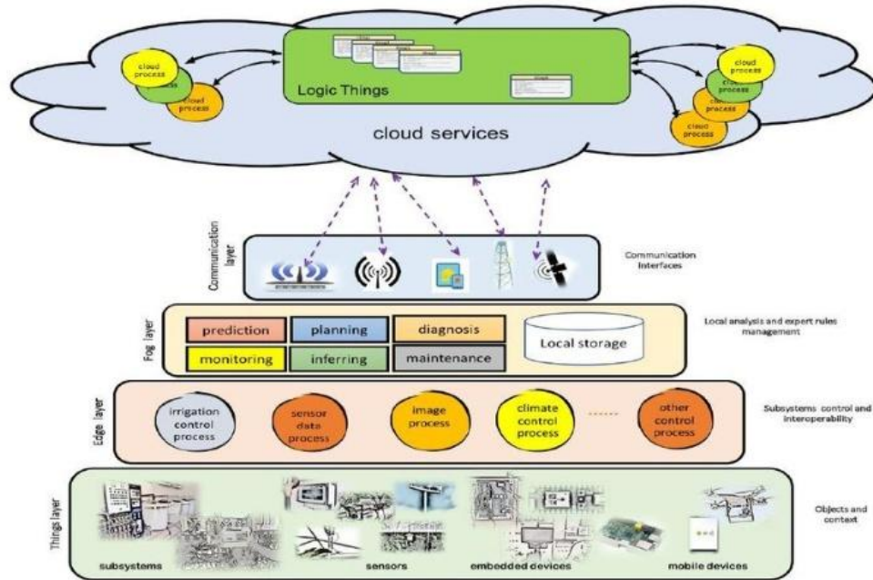
Fig 1: IoT based precision farming
