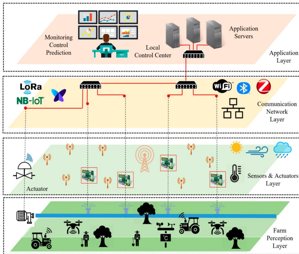
Fig 4: LoraWAN based approach
